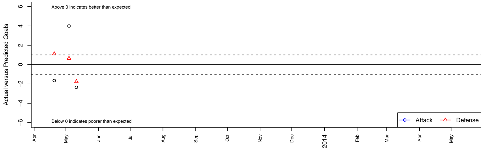
KVJSA Ellensburg FC B98 Dots are actual minus expected GF (blue circles) and GA (red triangles). Blue line is smoothed change in attack strength. Red is smoothed change in defense strength.
